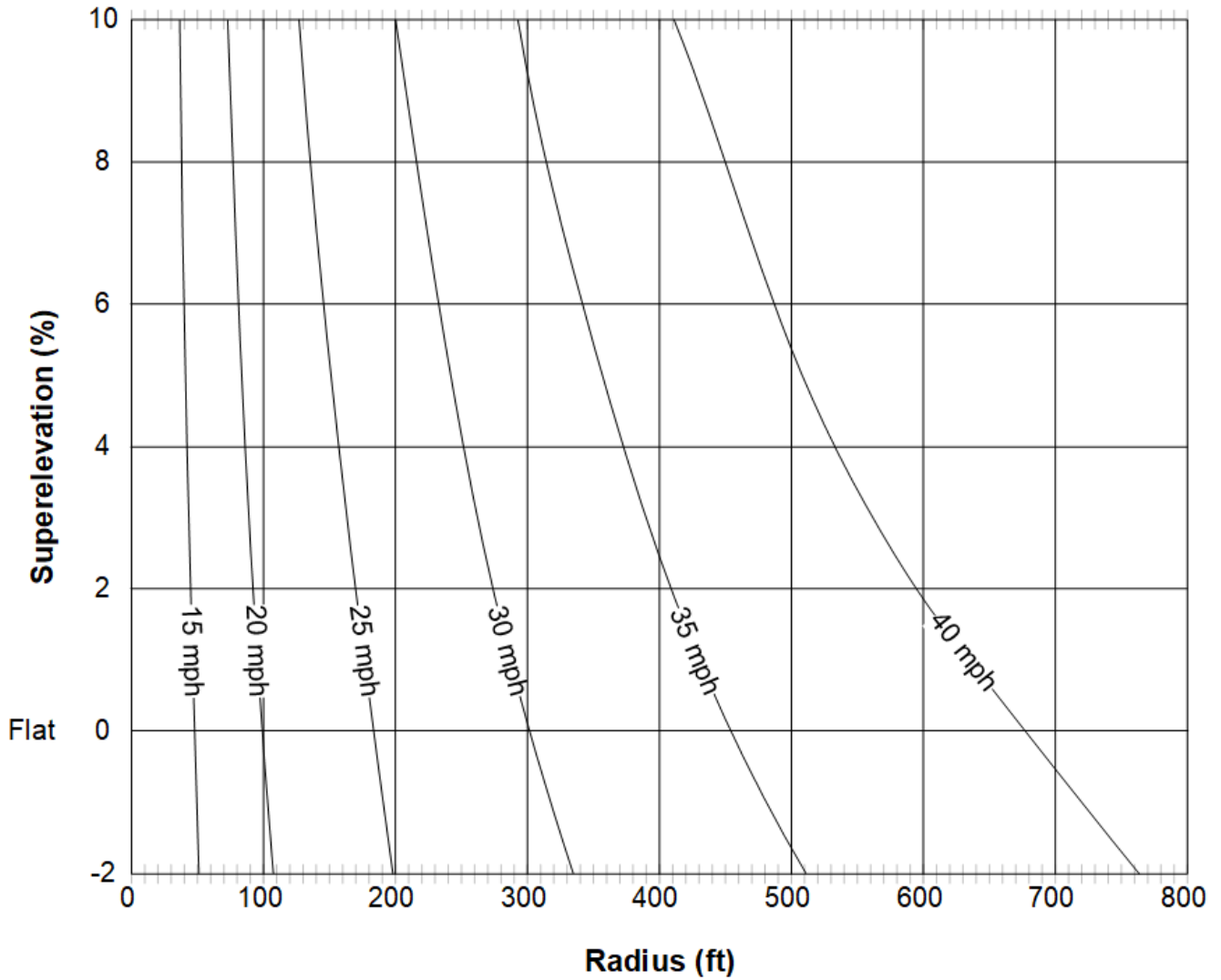
Exhibit 1250-7 Superelevation Rates for Low-Speed Streets in Urban Areas Where Speed is Relatively Low and Variable or at Intersections
