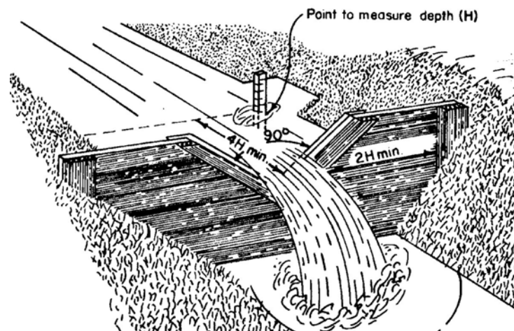
V-notch Weir
