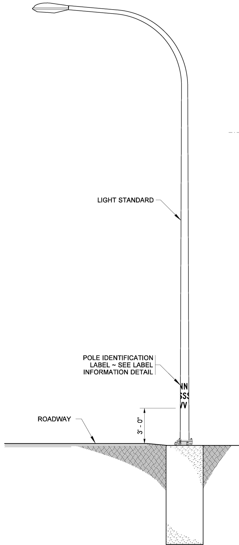
ELEVATION VIEW
