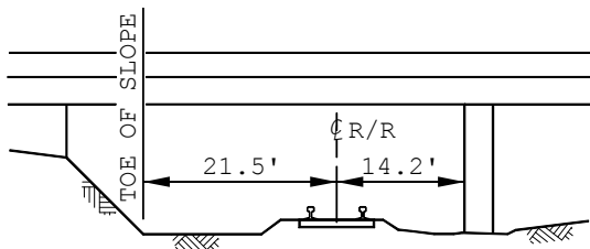
RAILROAD SINGLE TRACK
