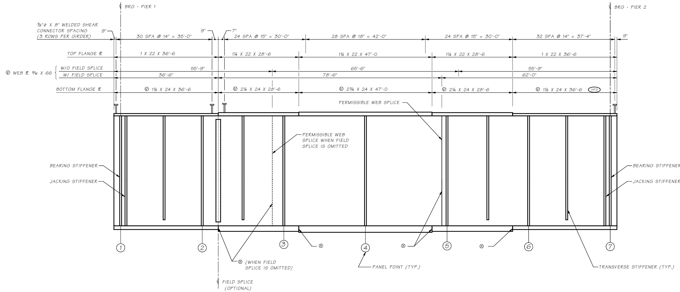
EXAMPLE - GIRDER ELEVATION
