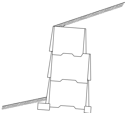
Precast Concrete Bin Wall
